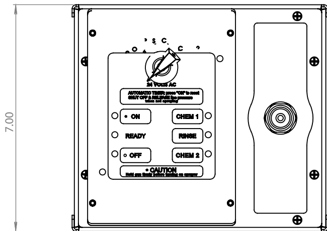
FRONT VIEW WITH TOUCHPAD OPTION
